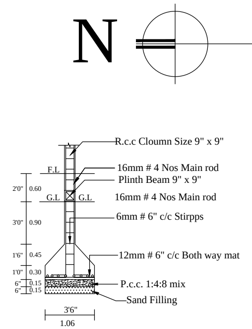
COLUMN DETIAL
