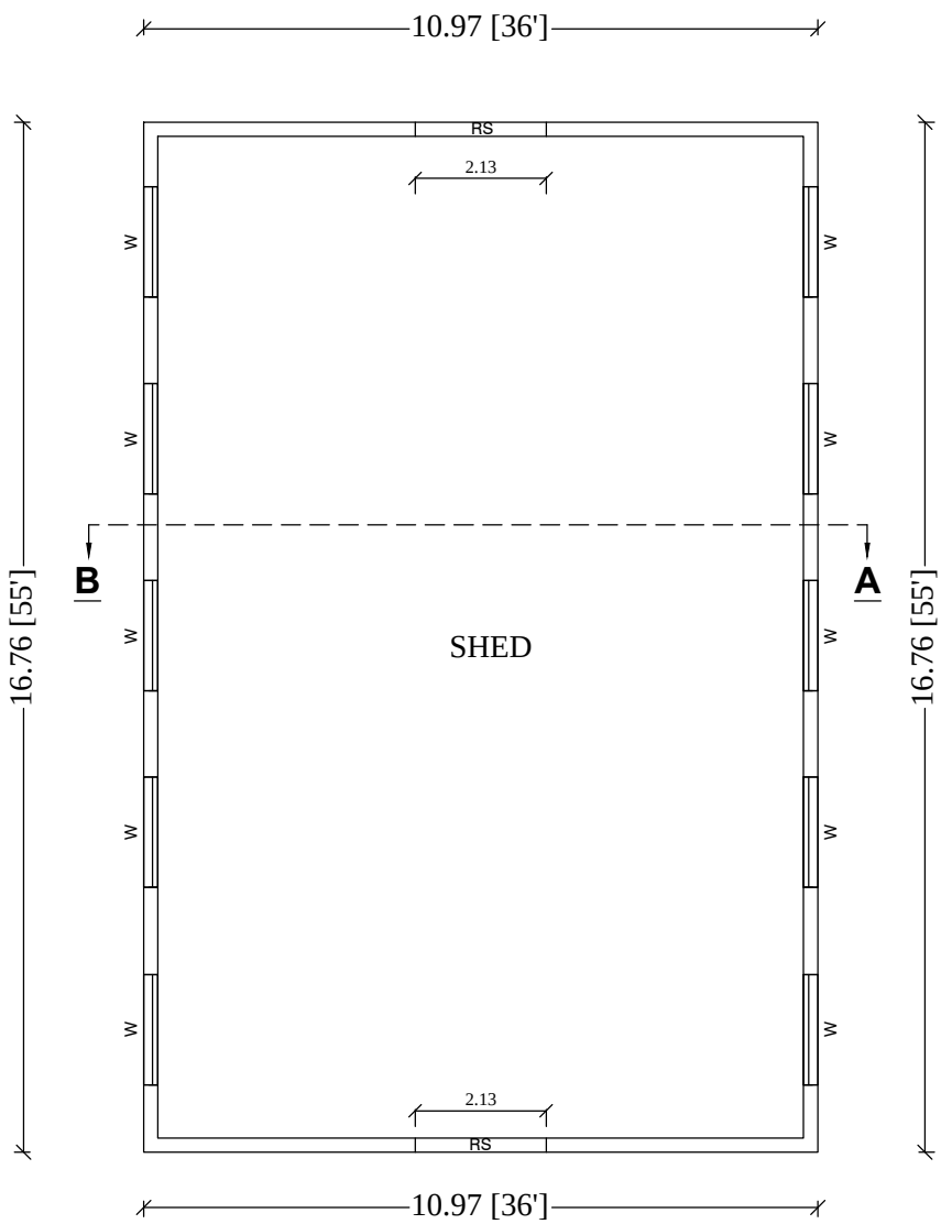
PLAN
