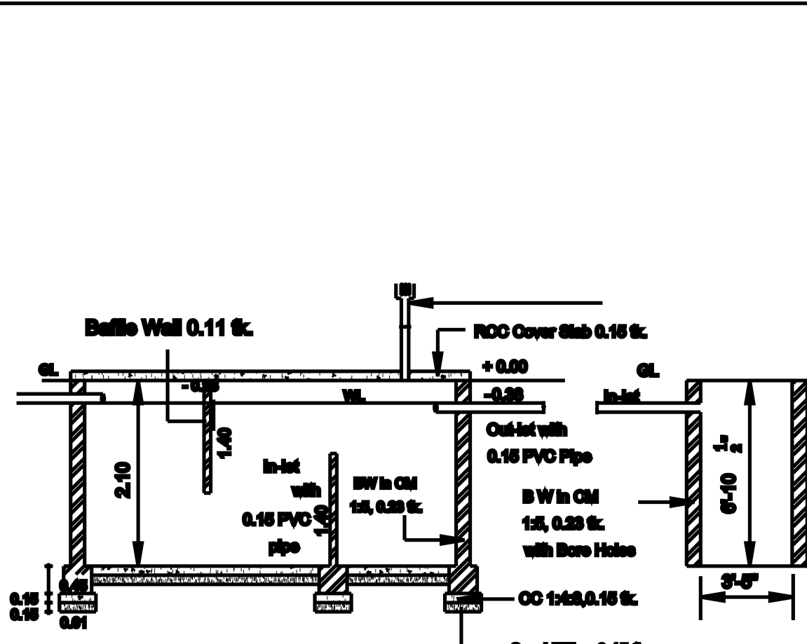
SECTION - SEPTIC TANK & SOAK PIT
