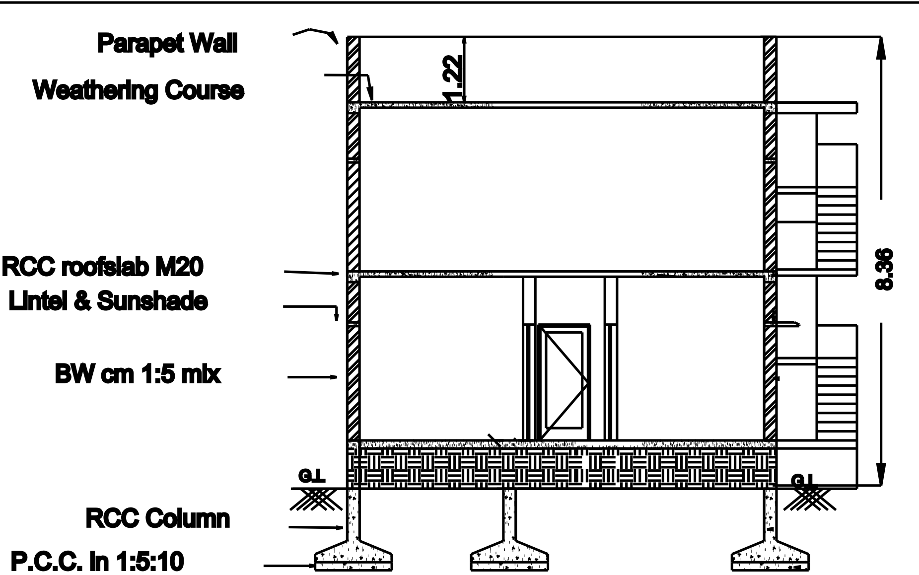
SECTION- BB
