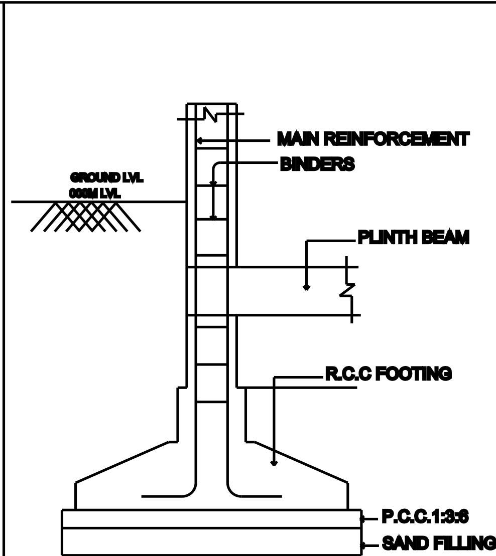
TYPICAL SECTION OF R.C.C COLUMN FOUNDATION
