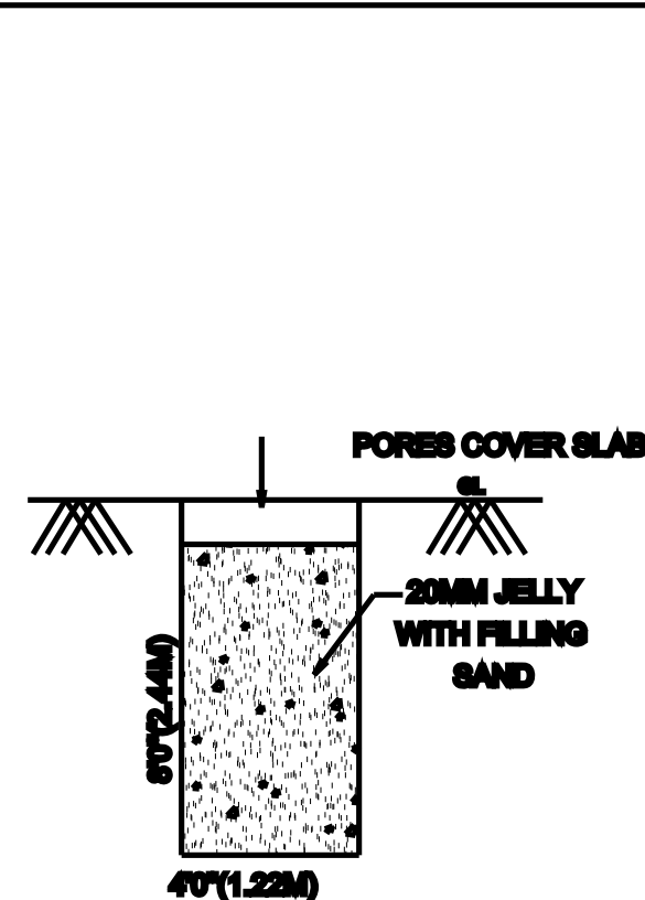
RAINWATER HARVESTING UNIT
