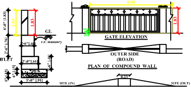
COMPOUND WALL & GATE DETAIL
