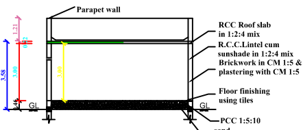
SECTION X - X
