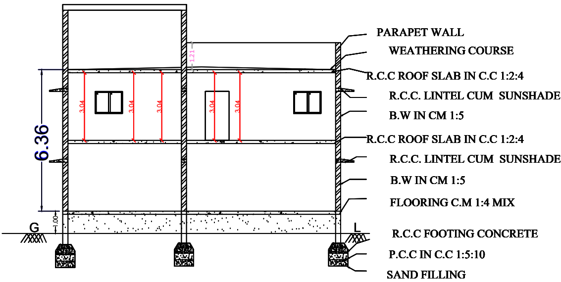
SECTION "AB"
