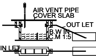
DETAILS OF SEPTIC TANK & D-TRENCH
