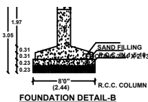
FOUNDATION DETAIL-B
