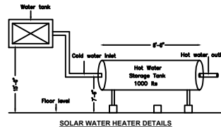
SOLAR WATER HEATER DETAILS
