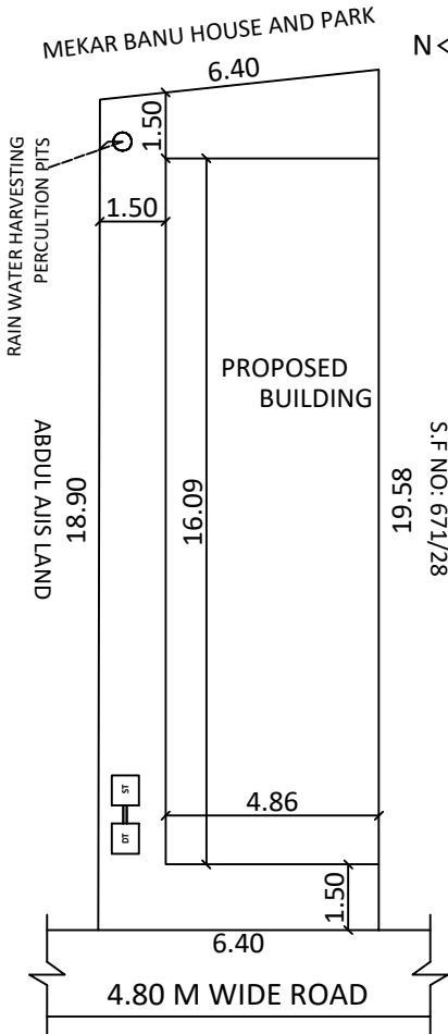
SITE PLAN
