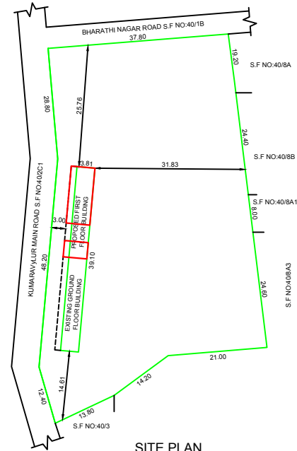
SITE PLAN SCALE 1:400.
