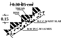
STAIRCASE SECTION
