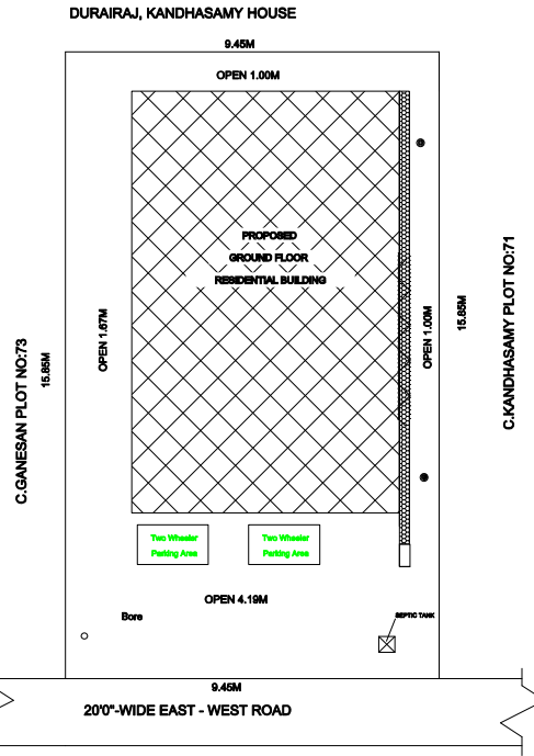
SITE PLAN (SCALE 1:1)
