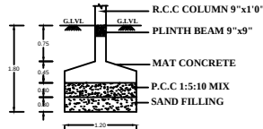
COLUMN FOUNDATION (NOT TO SCALE)
