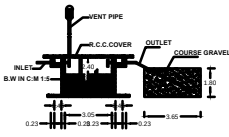
SEPTIC TANK & D-TRENCH DETAILS (NOT TO SCALE)
