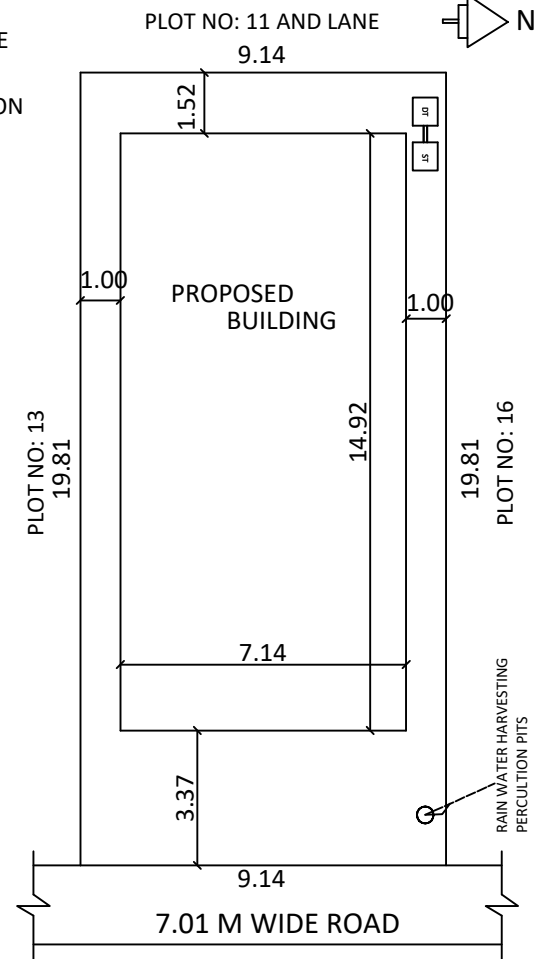
SCALE 1:100.
