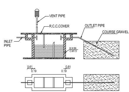
SEPTIC TANK & DISPERSION TRENCH DETAILS
