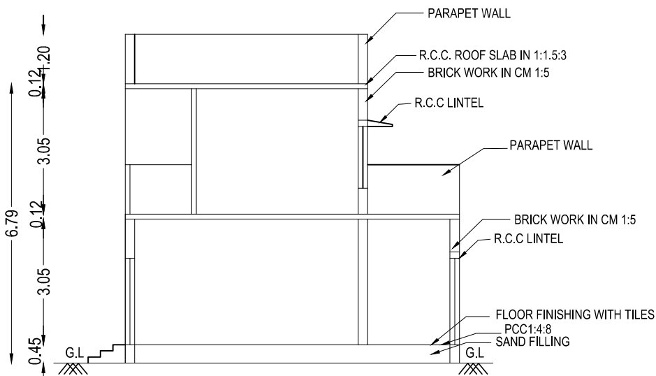
SECTION
