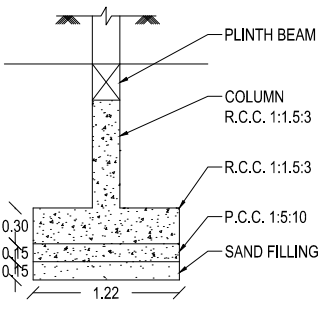
FOUNDATION DETAIL
