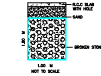
RAIN WATER HARVEST COLLECTION PIT.
