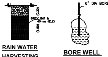
BORE WELL
