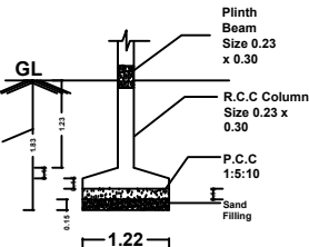
FOUNDATION DETAILS
