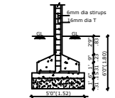
COLUMN FOUNDATION DETAIL
