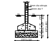
COLUMN FOUNDATION DETAIL
