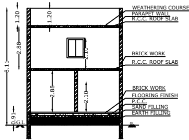
SECTION ON XX
