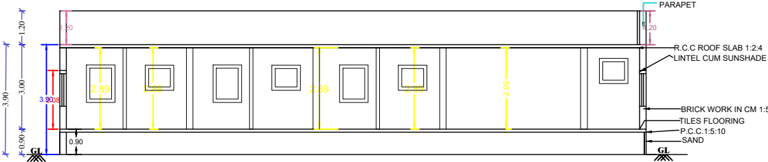
SECTION ON A-B
