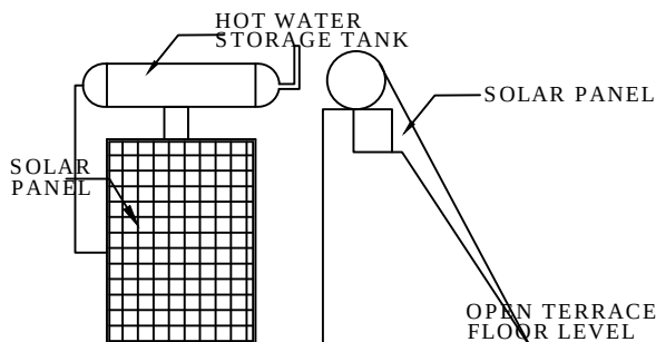
SOLAR SYSTEM DETAILS
