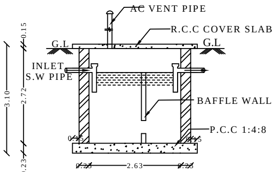
SAEPTIC TANK DETAILS
