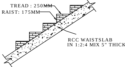
STAIRCASE DETAILS
