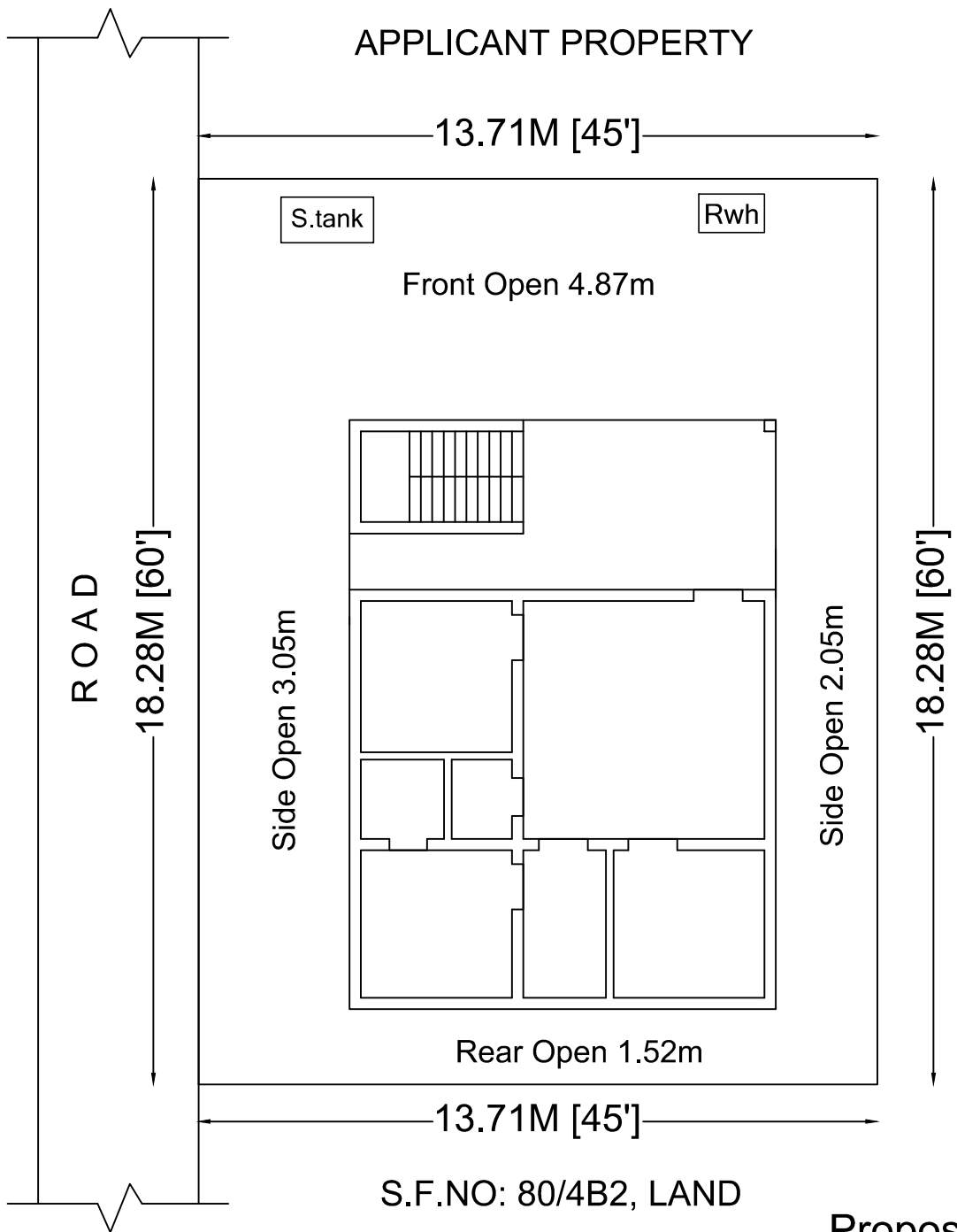
Proposed Site Plan SCALE 1:100
