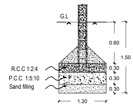
FOUNDATION DETAIL
