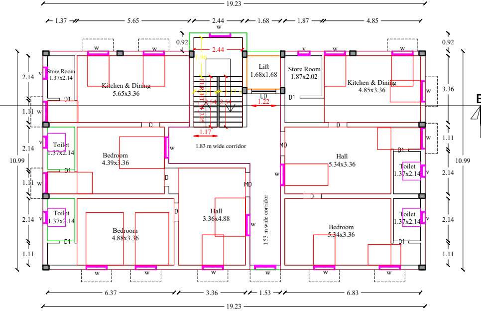
FIRST FLOOR PLAN TYPICAL_FLOOR_PLAN=1,2
