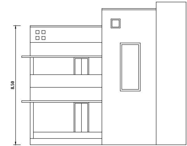
FRONT ELEVATION
