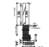
COMPOUND WALL
