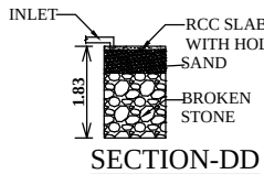
SECTION-DD
