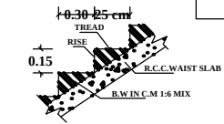
SECTION OF STAIRCASE
