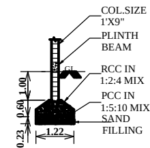
COLUMN DETAILS
