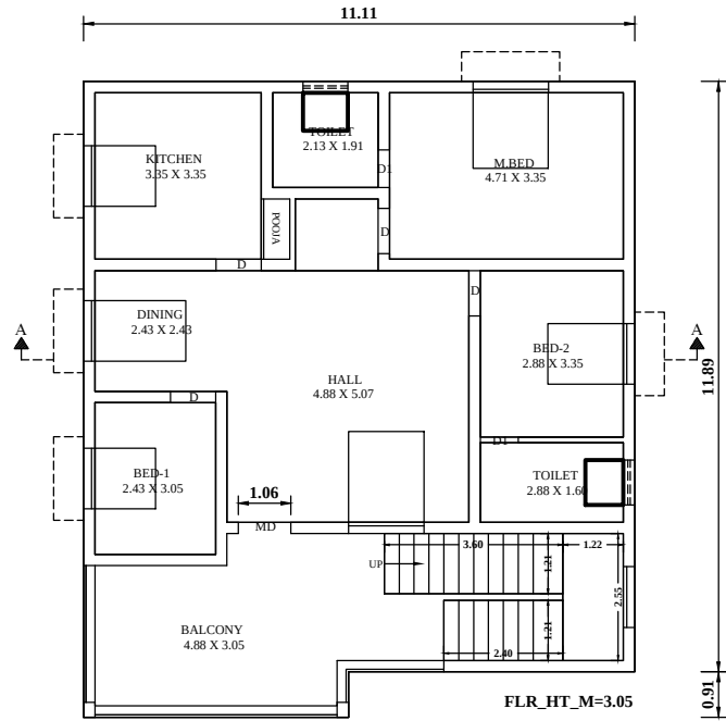
PRO FIRST FLOOR
