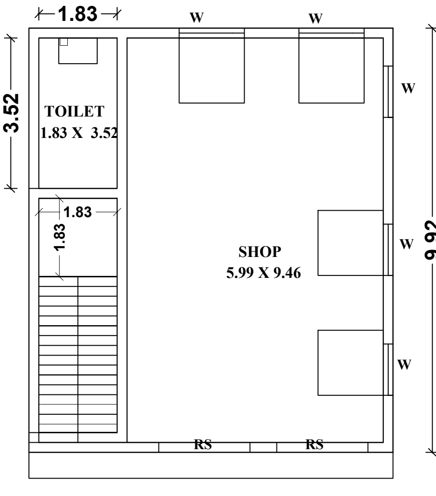
PRO.FIRST LOOR PLAN
