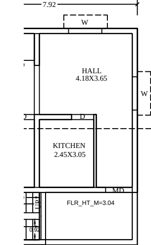
F.FLOOR PLAN
