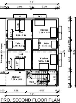
PRO. SECOND FLOOR PLAN
