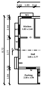
EXG. GROUND FLOOR PLAN
