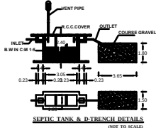
SEPTIC TANK & D-TRENCH DETAILS NOT TO SCALE
