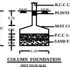
COLUMN FOUNDATION NOT TO SCALE
