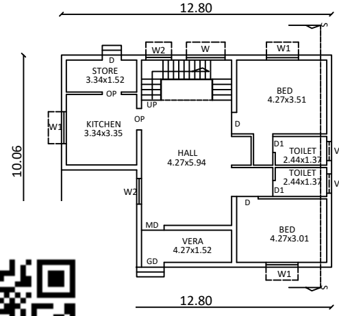
ND FLOOR PLAN
