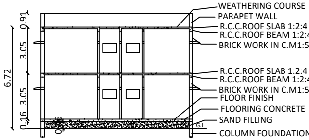
SECTION-SS
