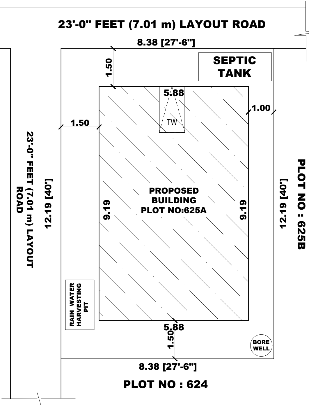
SITE PLAN
