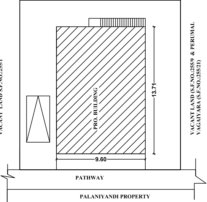
SITE PLAN
