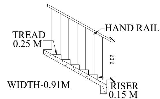
STAIRCASE DETAILS
