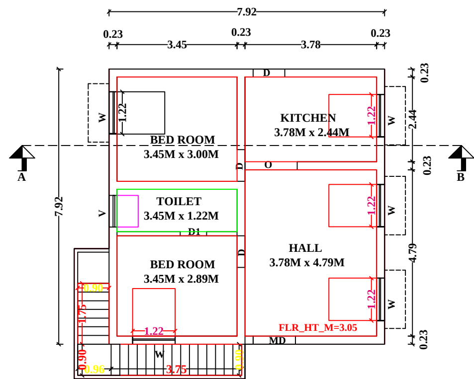
FLOOR-GROUND PRO.GROUND FLOOR PLAN
