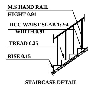
STAIRCASE DETAIL
