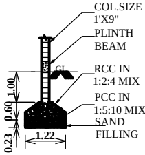
COLUMN DETAILS
