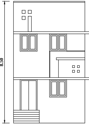
FRONT ELEVATION
