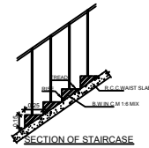
SECTION OF STAIRCASE
