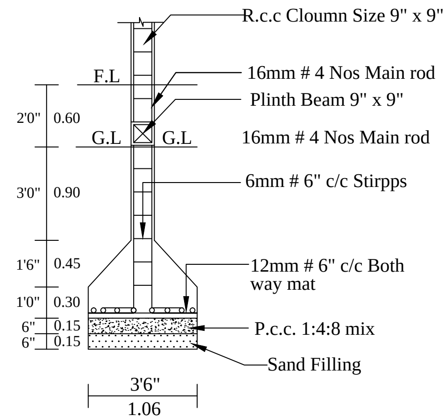
COLUMN DETIALS
