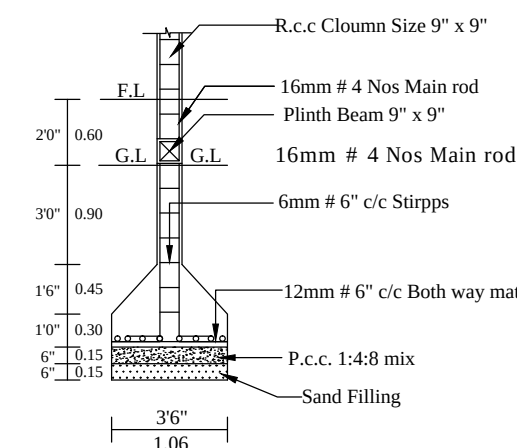
COLUMN DETIAL
