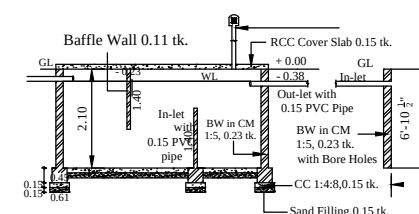
SECTION - SEPTIC TANK &amp; SOAK PIT
