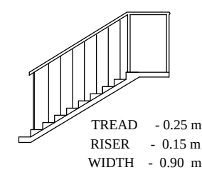
STAIRCASE DETAILS
