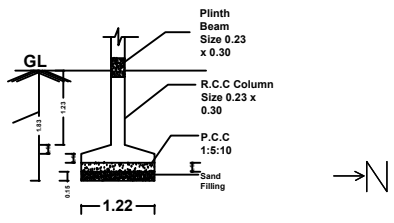
FOUNDATION DETAILS
