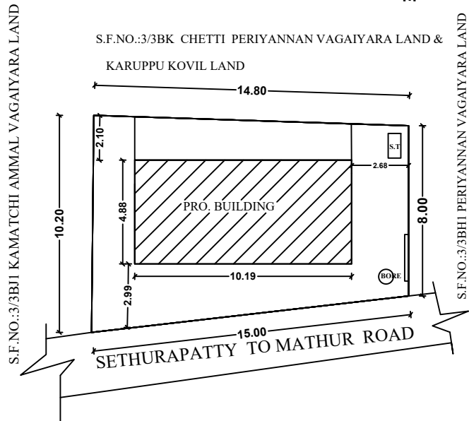
SITE PLAN
