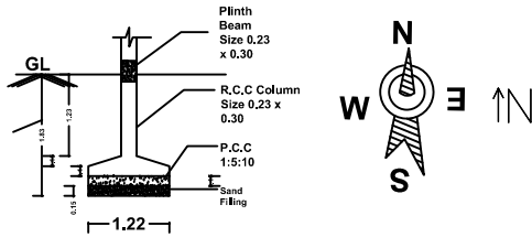
FOUNDATION DETAILS
