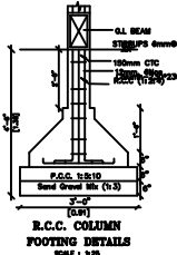
R.C.C. COLUMN FOOTING DETAILS SCALE : 1:25
