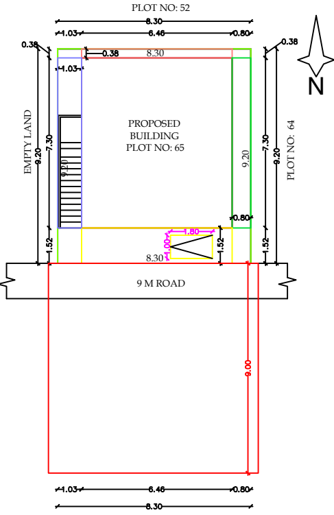
SITE PLAN
