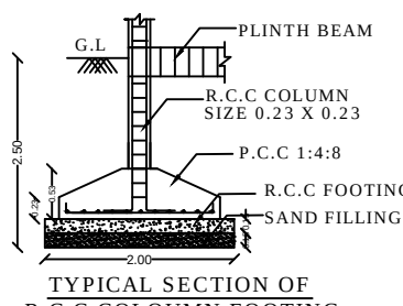
TYPICAL SECTION OF R.C.C COLOUMN FOOTING
