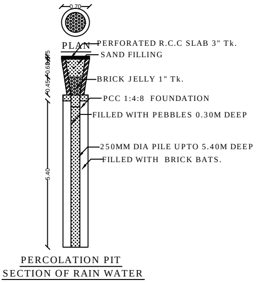
PERCOLATION PIT SECTION OF RAIN WATER
