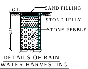
DETAILS OF RAIN WATER HARVESTING
