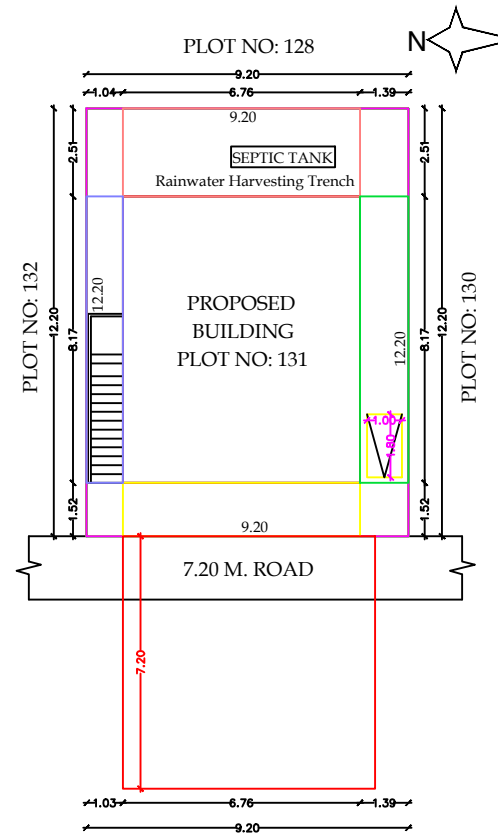
SITE PLAN
