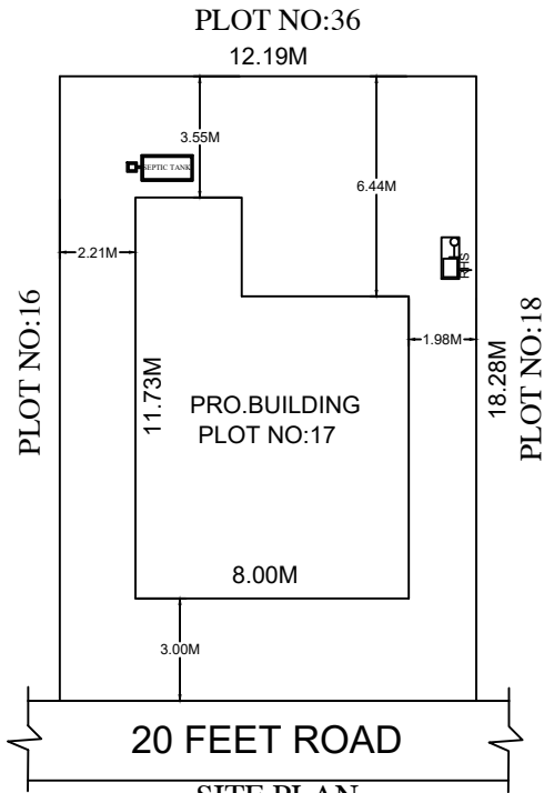
SITE PLAN
