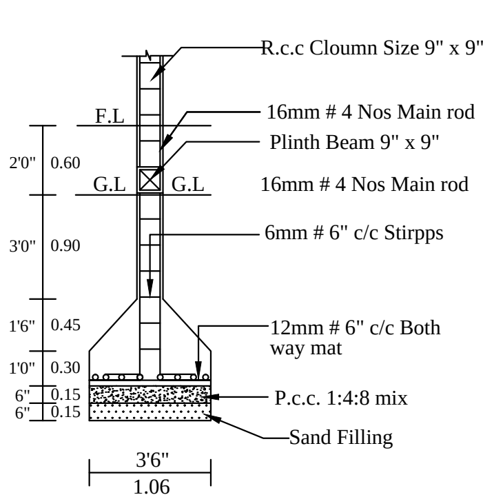
COLUMN DETIALS
