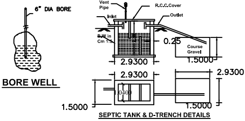
SEPTIC TANK & D-TRENCH DETAILS
