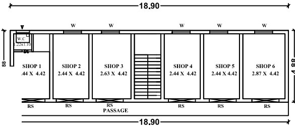
PRO.FIRST FLOOR PLAN
