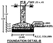
FOUNDATION DETAIL-B
