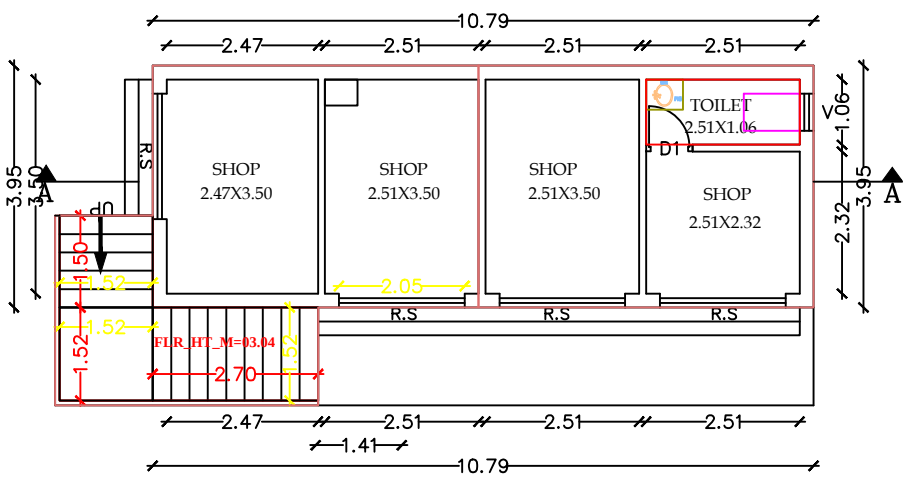
EXISTING & PROPOSED GROUND FLOOR PLAN
