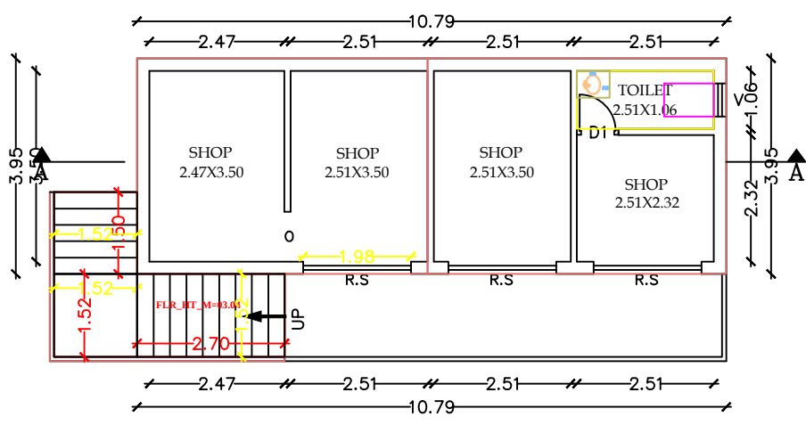
EXISTING & PROPOSED FIRST FLOOR PLAN
