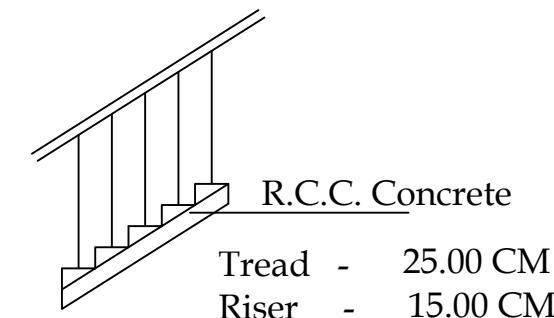
Staircase details
