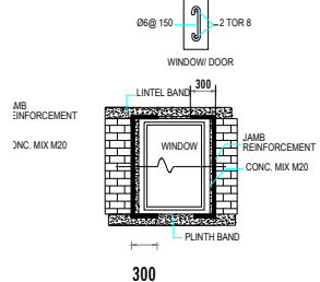
DETAILS OF OPENINGS
