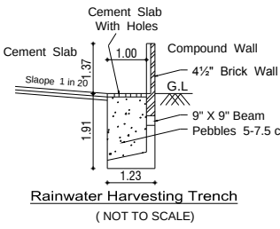
Rainwater Harvesting Trench
