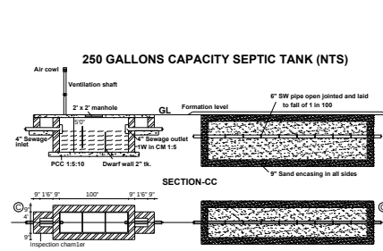
250 GALLONS CAPACITY SEPTIC TANK (NTS)
