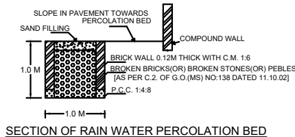
SECTION OF RAIN WATER PERCOLATION BED
