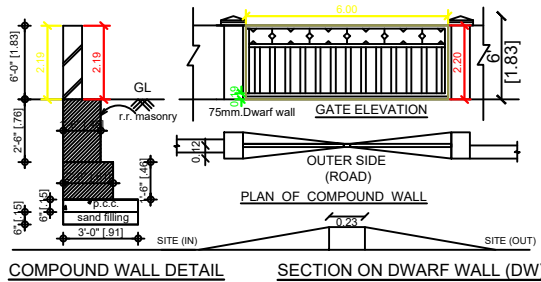
COMPOUND WALL DETAIL
