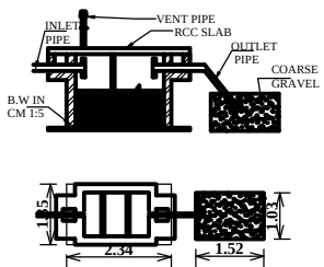
SEPTIC TANK & D-TRENCH DETAILS (NOT TO SCALE)
