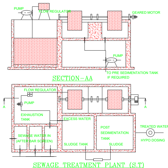
SEWAGE TREATMENT PLANT (S.T)
