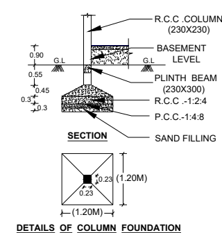
DETAILS OF COLUMN FOUNDATION
