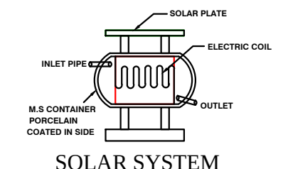
SOLAR SYSTEM
