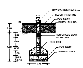
FOUNDATION DETAILS
