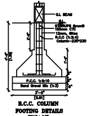
R.C.C. COLUMN FOOTING DETAILS SCALE 1:100
