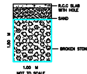
RAIN WATER HARVEST COLLECTION PIT. NOT TO SCALE
