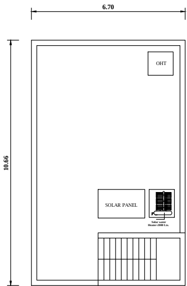
GROUND FLOOR ROOF PLAN
