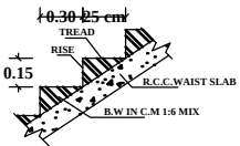
SECTION OF STAIRCASE
