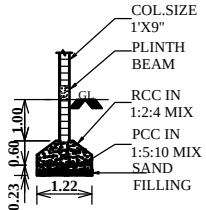
COLUMN DETAILS
